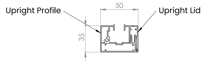
ART 110 Upright Profiles
