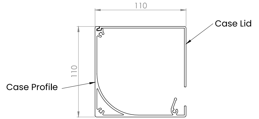
ART 110 Case Profiles
